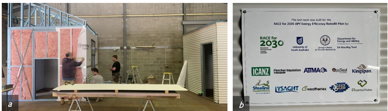
Figure 11. (a) Two 3 m x 3 m test rooms were built in Adelaide, mimicking the construction of houses in the APY Lands. (b) They were made possible through the support of industry partners and donors of materials: ICANZ, Fletcher Insulation, ATMA, OptiSeal, Kingspan, Steeline Mt Gambier, Lysaght, Weathertex, Neata Glass, and Efficiency Matrix.
