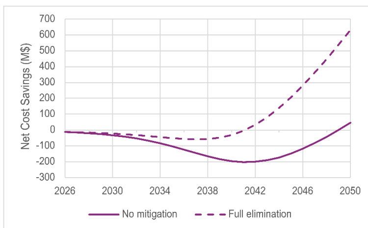
Figure 22. Comparison of net cost savings nationally between non-mitigated and fully mitigated linear thermal bridges, under modest adoption rates for a level 3 retrofit. These two curves represent likely lower and upper limits of the direct economic benefit.
